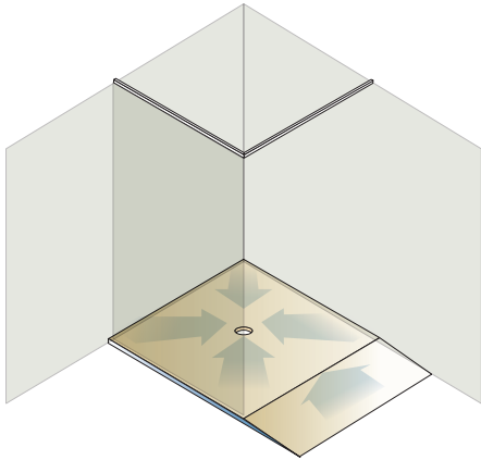
1m x 1m Tray + 300mm Ramp & Glass Panel
